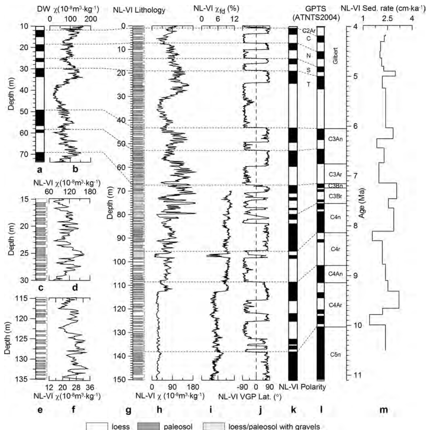
Figure 6. Magnetostatigraphy, magnetic susceptibility and sedimentation rate of NL-VI and correlations with the geomagnetic polarity timescale (GPTS). (a) Magnetic polarity of the Dongwan (DW) section (Hao & Guo 2004); (b) magnetic susceptibility of the Dongwan section (Hao & Guo 2004) and correlation with NL-VI; (c–d and e–f) zoomed lithology columns and magnetic susceptibility of NL-VI; (g) lithology of NL-VI; (h) magnetic susceptibility of NL-VI; (i) frequency dependent magnetic susceptibility of NL-VI; (j) VGP latitude of NL-VI; (k) magnetic polarity of NL-VI; (l) ATNTS2004 GPTS (Gradstein et al. 2004) and (m) sedimentation rate of NL-VI.
